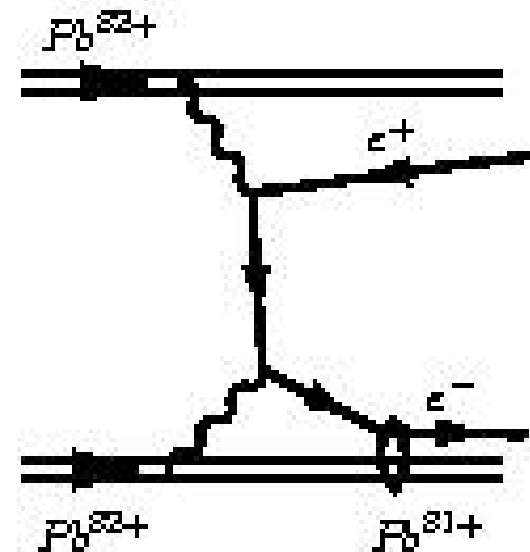
bound-free pair production
