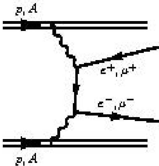
pair production
